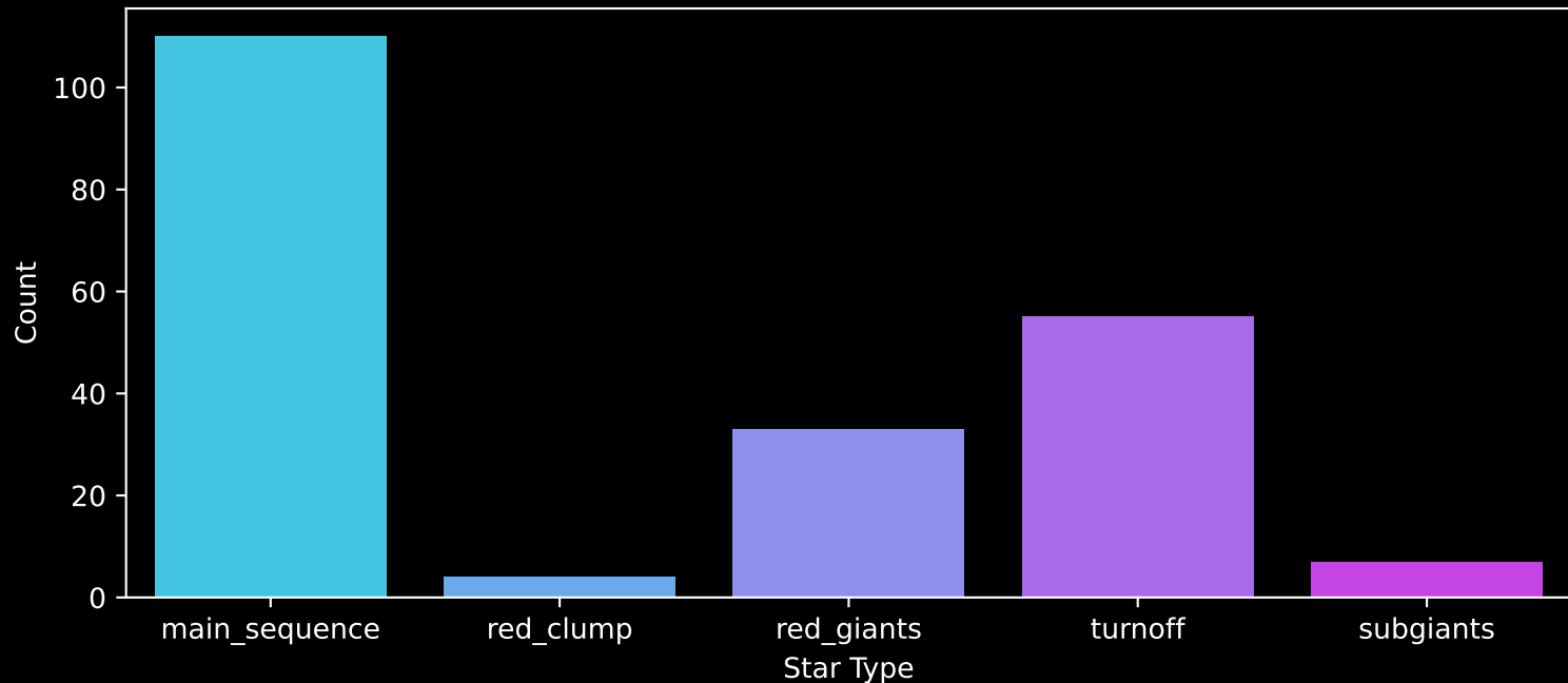
APOGEE DR17 Field: [284-39] Count plot of Star Type
