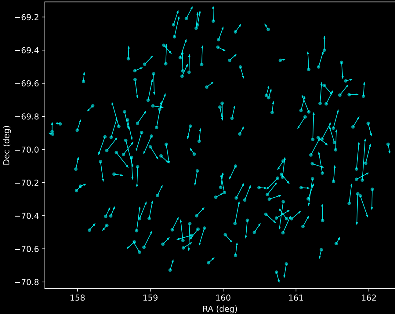
APOGEE DR17 Noise Stream Proper Motion Vectors (n=159)
