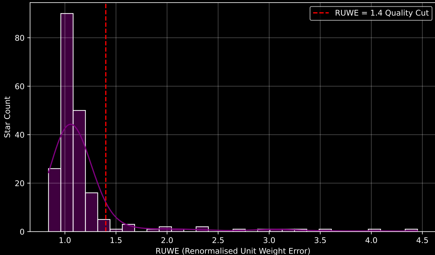
GAPOGEE DR17 Field [284-39] RUWE Distribution (n= 205)
