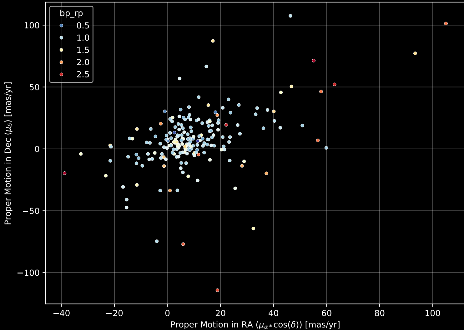
APOGEE DR17 Field: [284-39] Proper Motion Diagram (n= 209)
