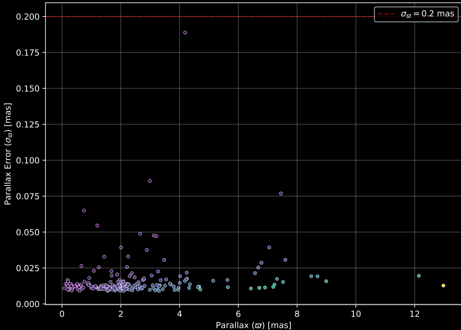
APOGEE DR17 Field: [284-39] Parallax Quality (n= 209)
